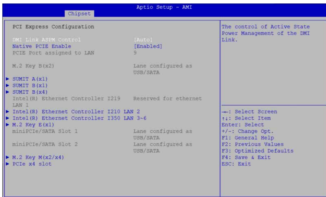
Figure 4-4-2-1 : PCH-IO Settings
