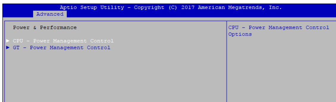
Figure 4 3-2 : Power & Performance
