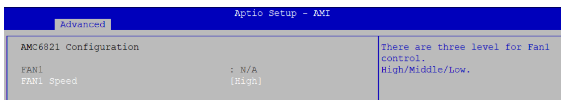
Figure 4-3-14 : AMC6821 Settings
