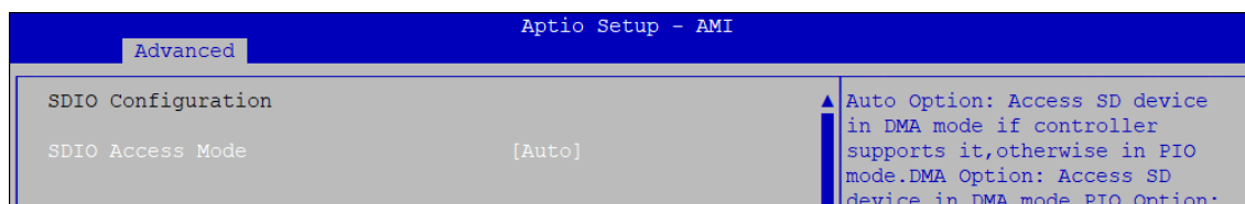
Figure 4-3-18 : SDIO Settings
