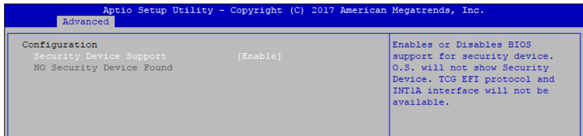
Figure 4 3-4 : Trusted Computing
